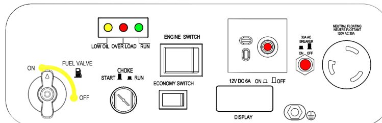
Figure 2. Control Panels
