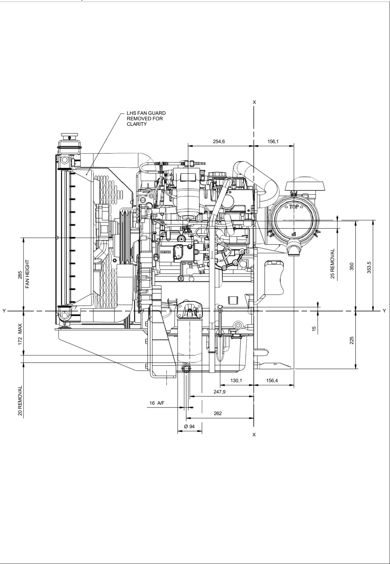
1103A-33TG2 ElectropaK - left view
